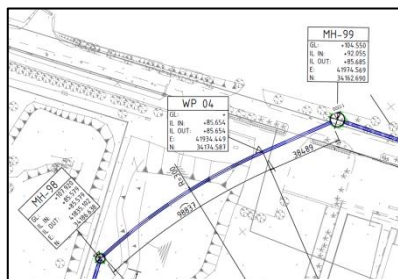
SITUATION: MH99 – MH98
